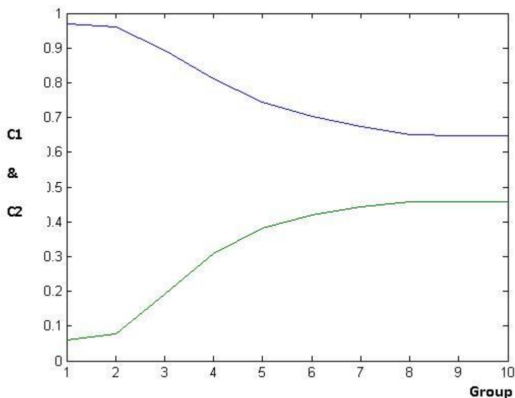
Figure 1.2: Closeness Measures
